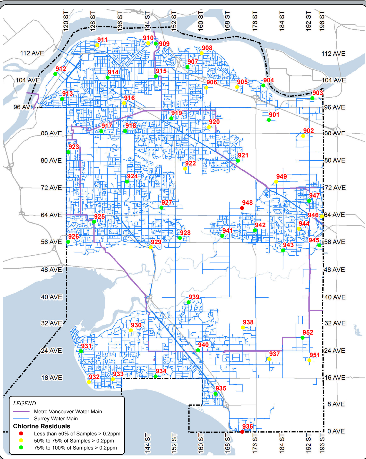
Fig. 5: CHLORINE RESIDUALS
