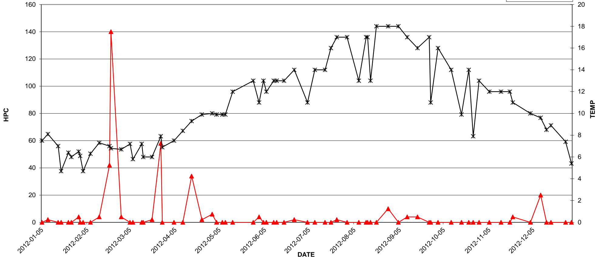
DM906 (SE CORNER 161 ST. & 102 AVE.) - 2012 TEST RESULTS
