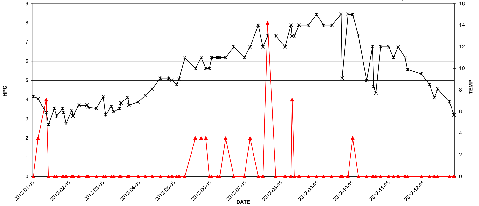
DM919 (NW CORNER 92A AVE. & 151 ST.) - 2012 TEST RESULTS
