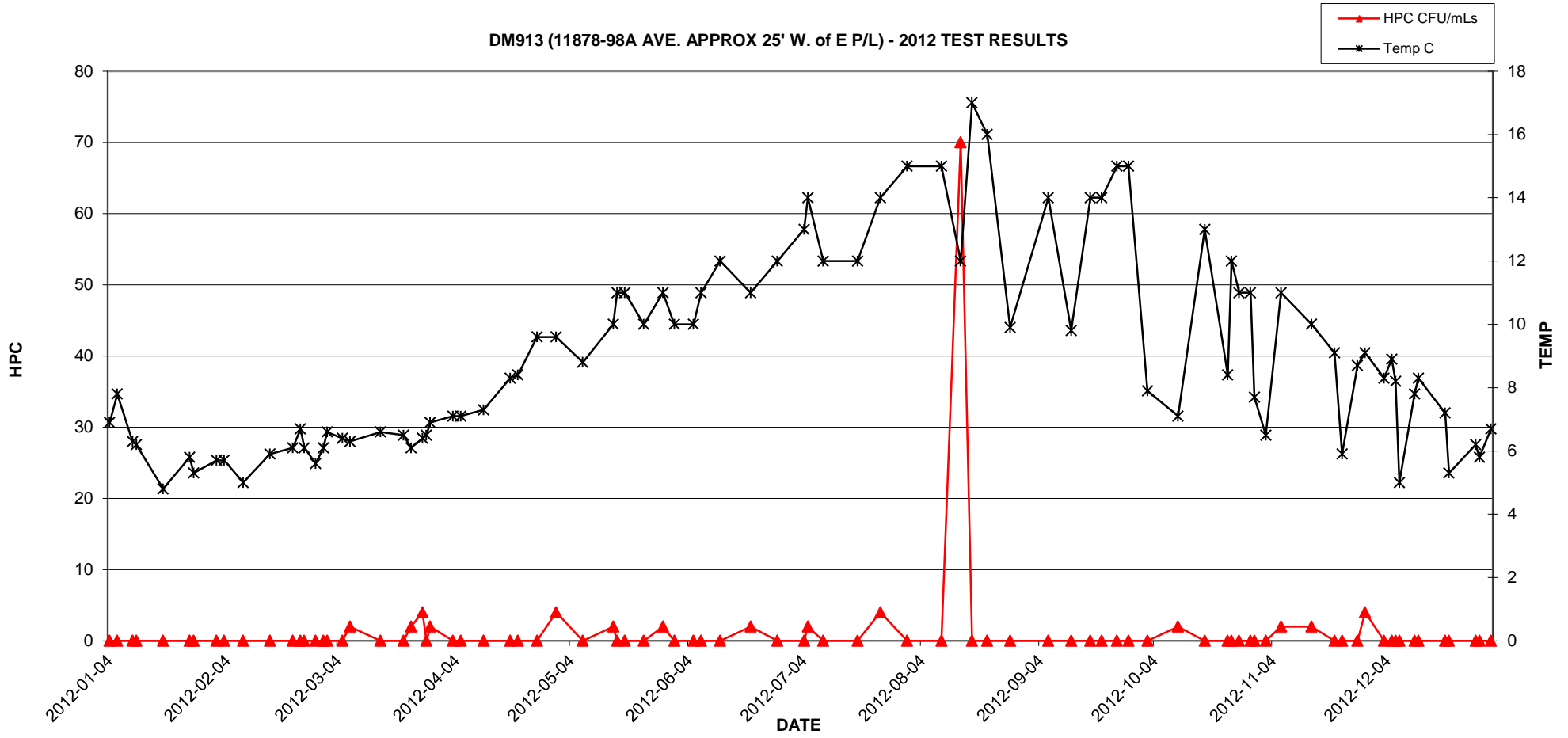
DM913 (11878-98A AVE. APPROX 25' W. of E P/L) - 2012 TEST RESULTS
