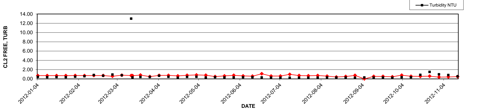
DM940 (SOUTHSIDE 24 AVE. at S DEPOT) - 2012 TEST RESULTS
