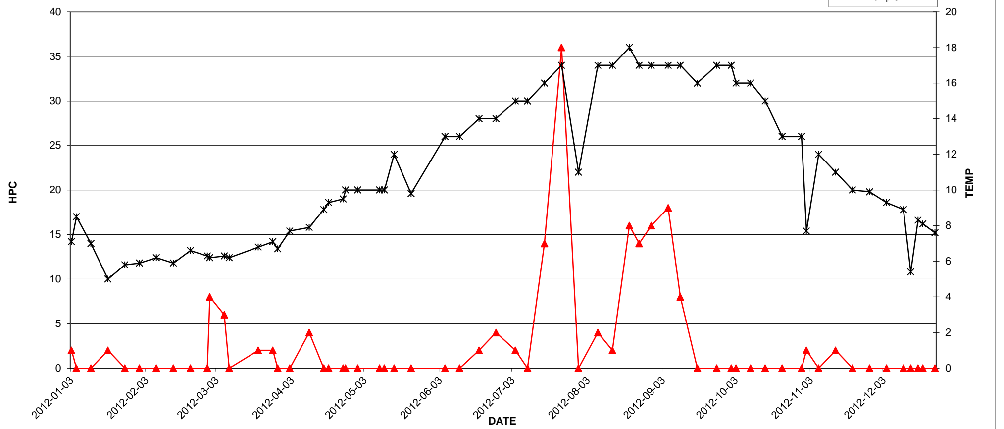
DM905 (SE CORNER 170A ST. & 102 AVE.) - 2012 TEST RESULTS
