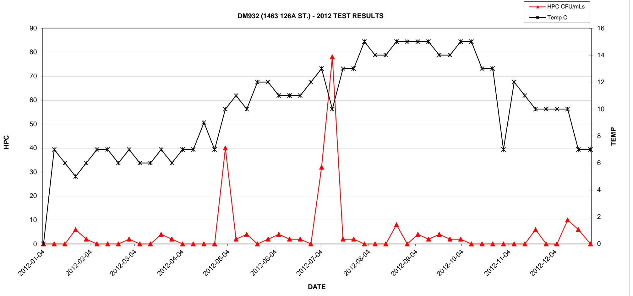
DM932 (1463 126A ST.) - 2012 TEST RESULTS
