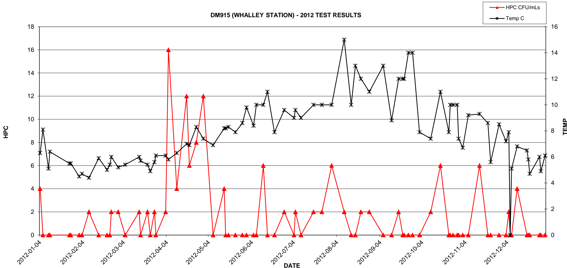
DM915 (WHALLEY STATION) - 2012 TEST RESULTS
