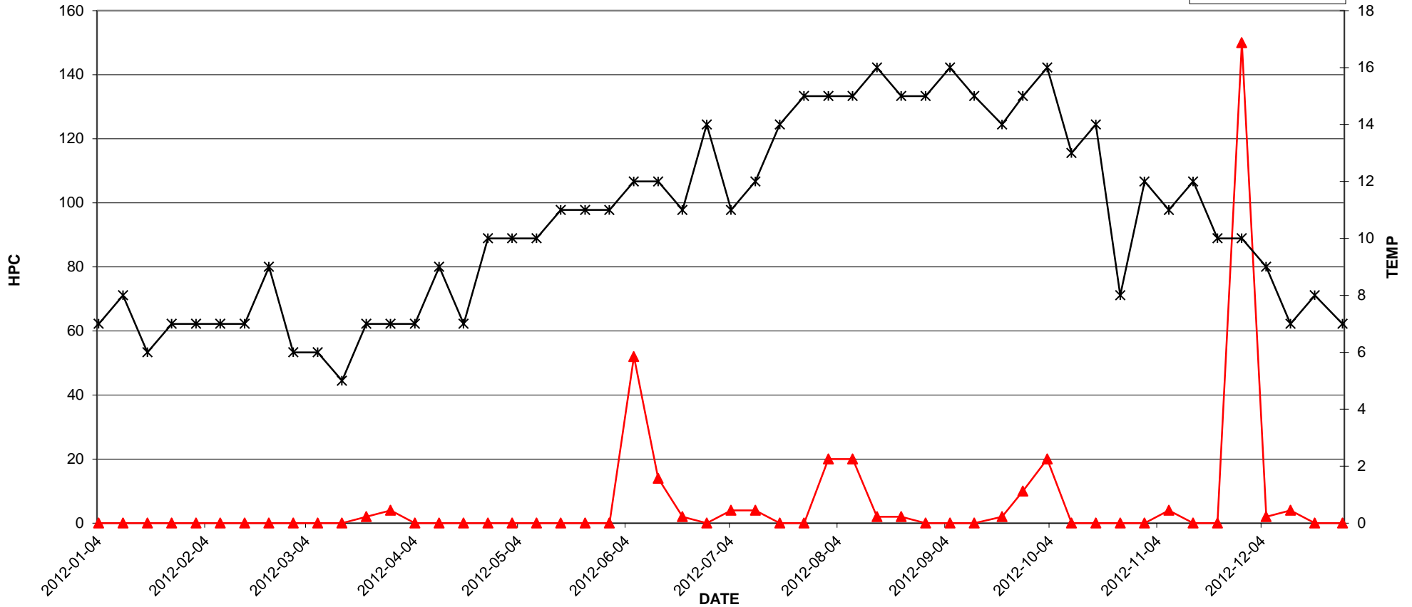
DM937 (NE CORNER 21A AVE. at 180 ST.) - 2012 TEST RESULTS
