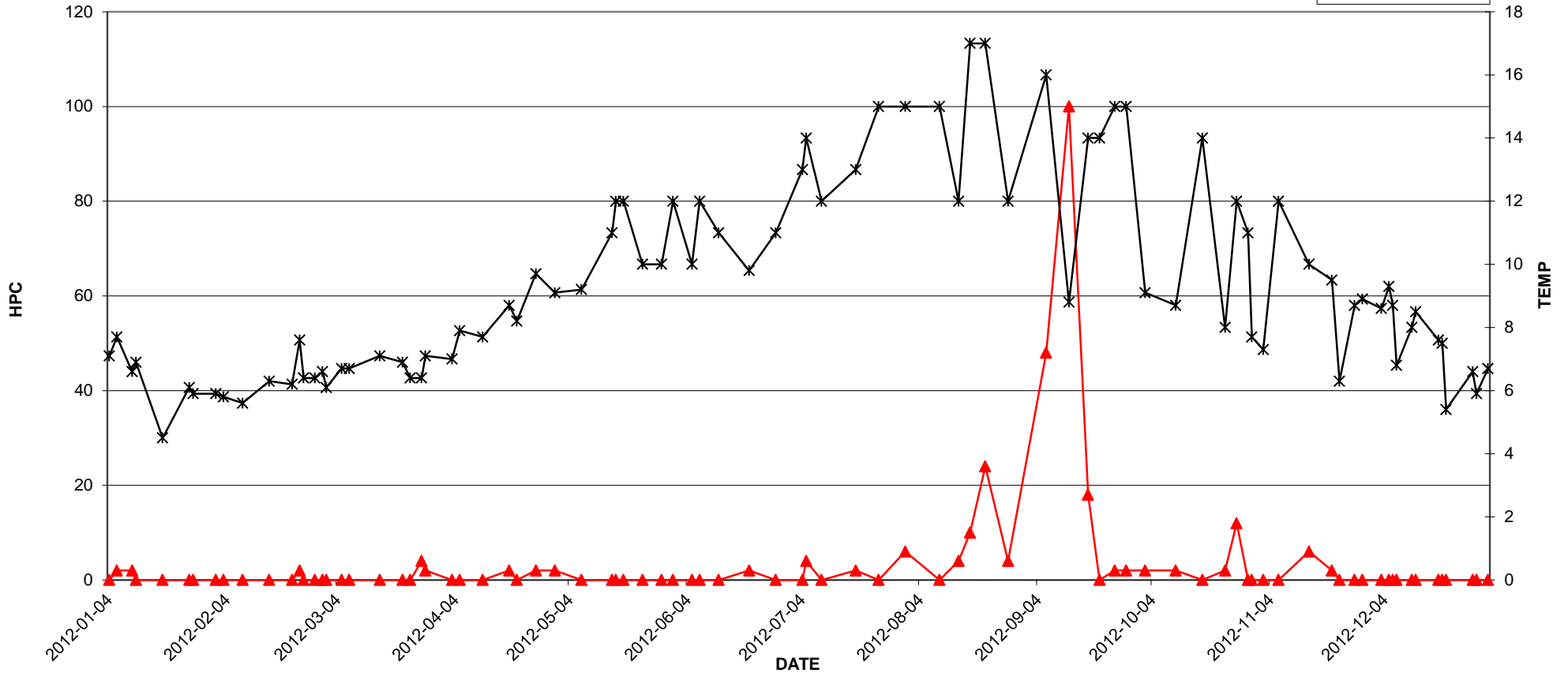
DM917 (E P/L 13031 Lanark PI.) - 2012 TEST RESULTS
