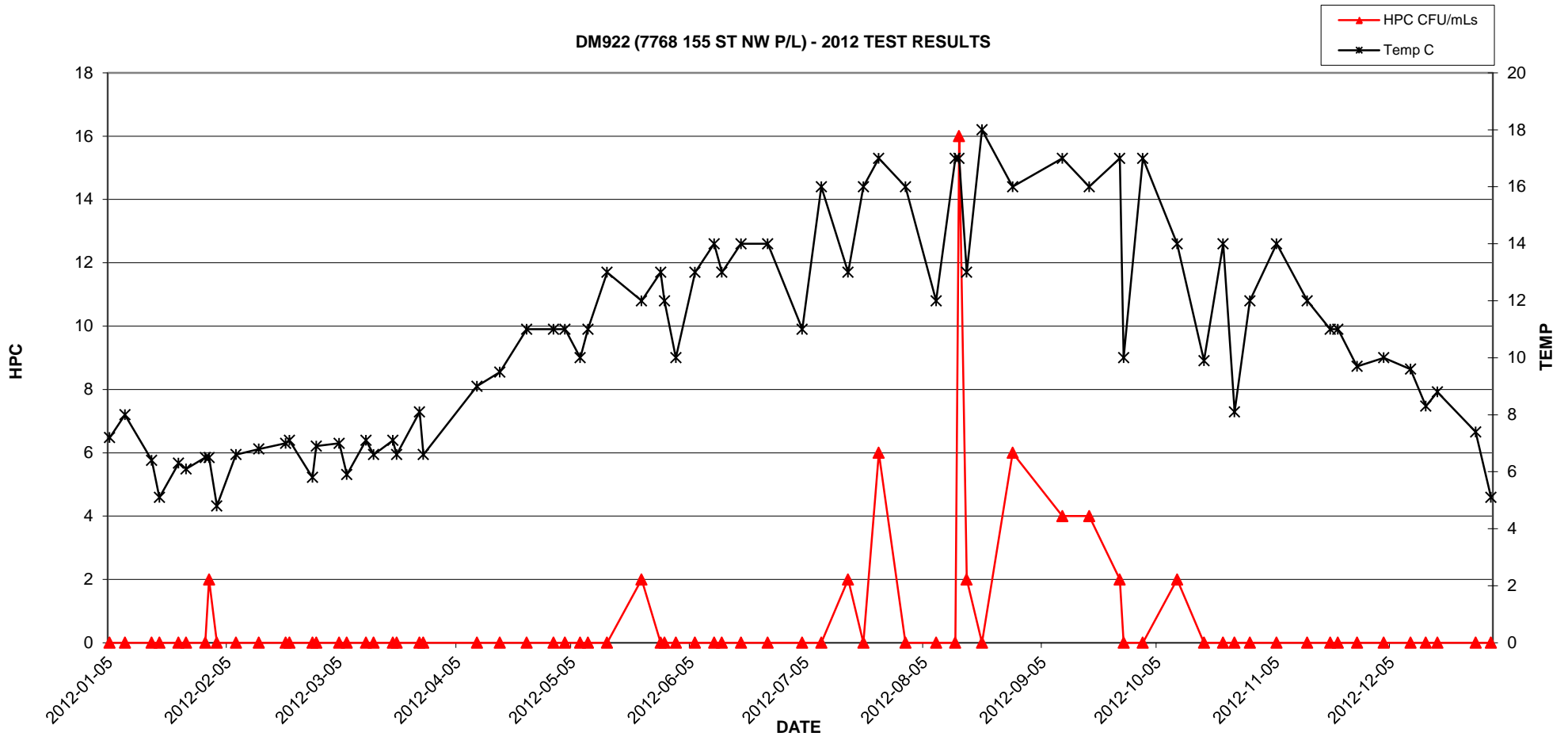
DM922 (7768 155 ST NW P/L) - 2012 TEST RESULTS
