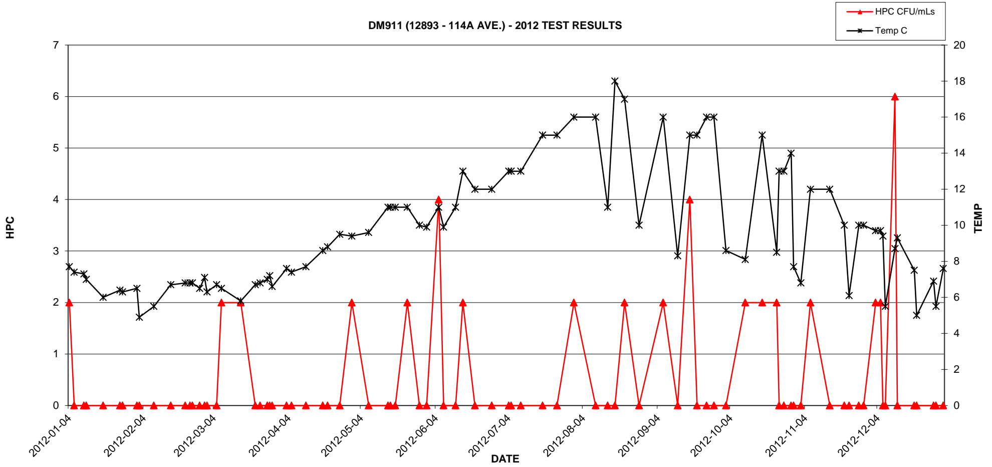
DM911 (12893 - 114A AVE.) - 2012 TEST RESULTS
