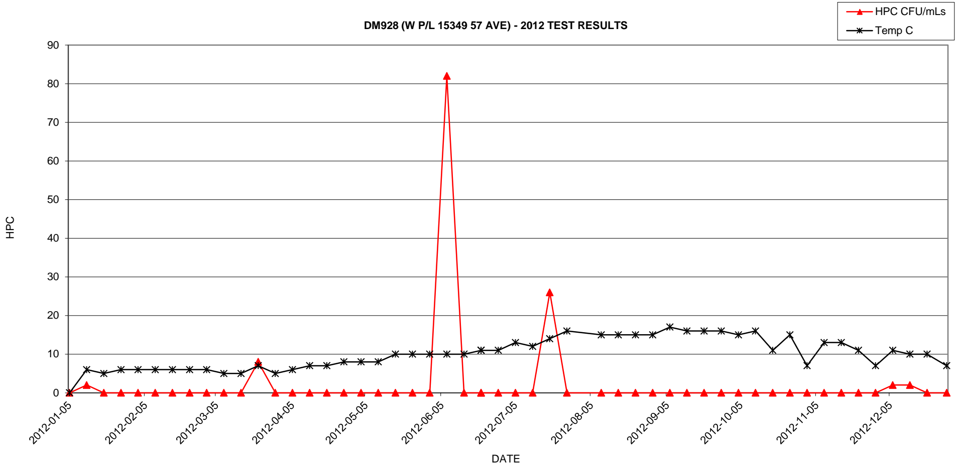
DM928 (W P/L 15349 57 AVE) - 2012 TEST RESULTS
