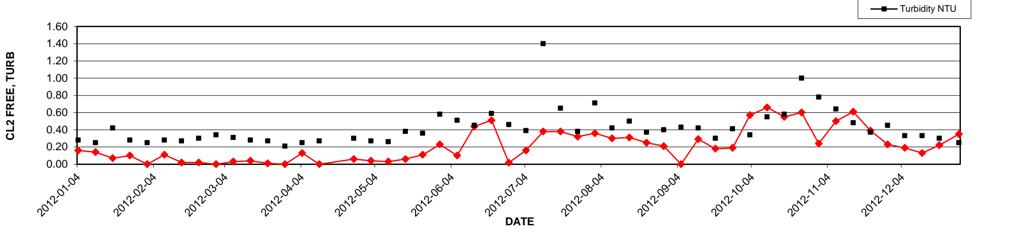
DM931 (SW CORNER 124 ST. and 24 AVE.) - 2012 TEST RESULTS
