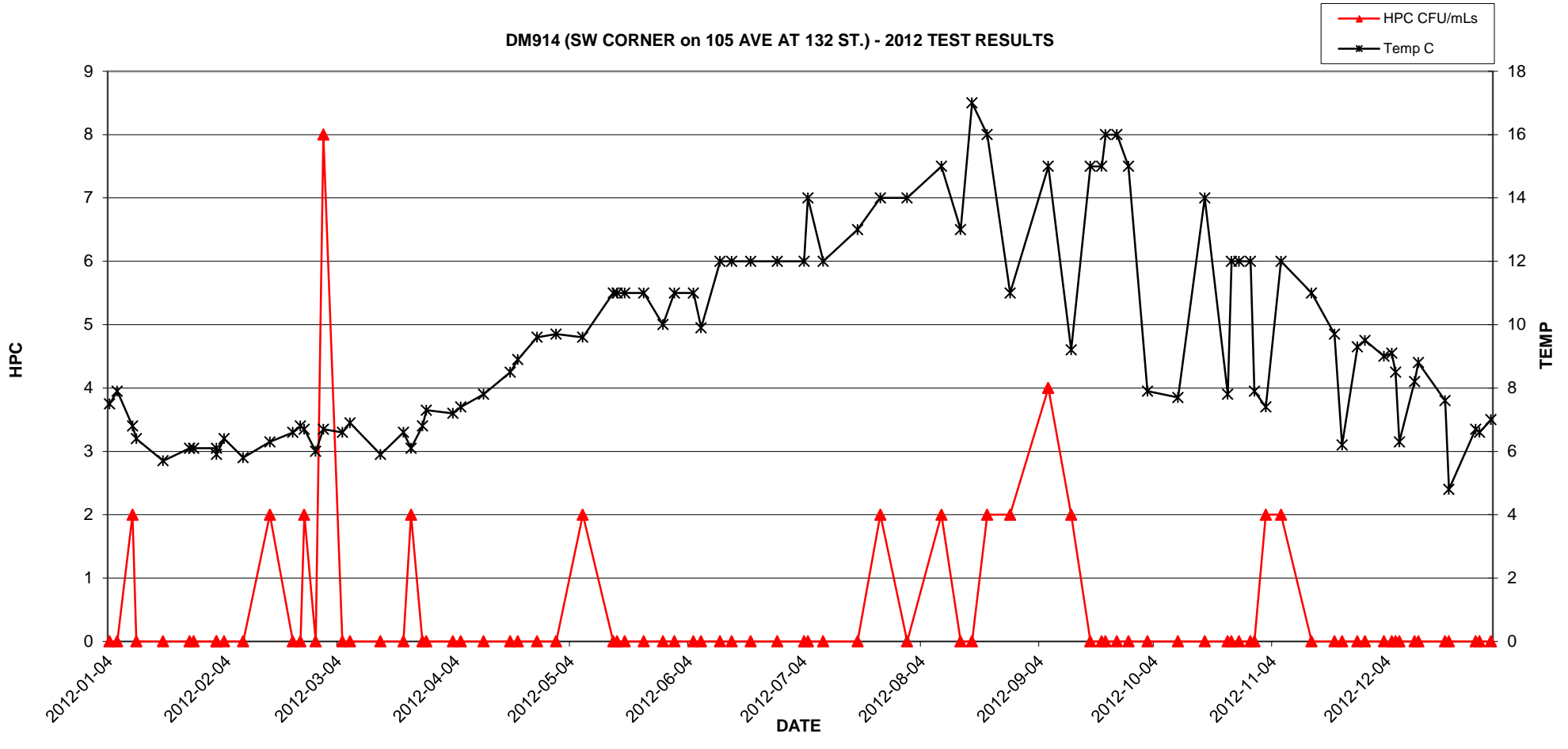
DM914 (SW CORNER on 105 AVE AT 132 ST.) - 2012 TEST RESULTS
