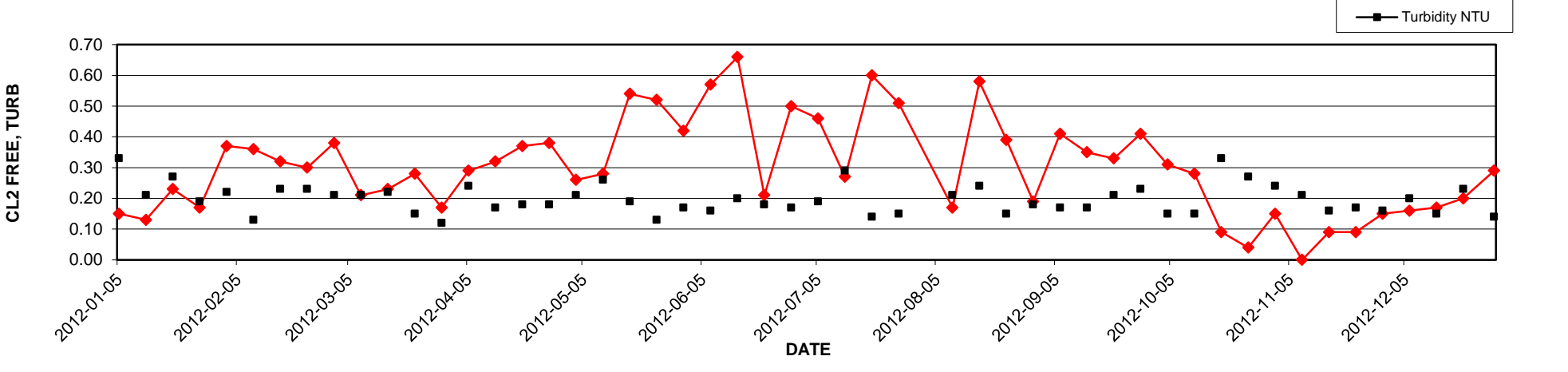
DM929 (SE LOMBARD PLACE at 144A ST.) - 2012 TEST RESULTS
