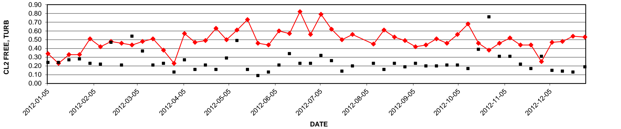
DM927 (CITY WORKS YARD - 66A AVE. AND 148ST.) - 2012 TEST RESULTS
