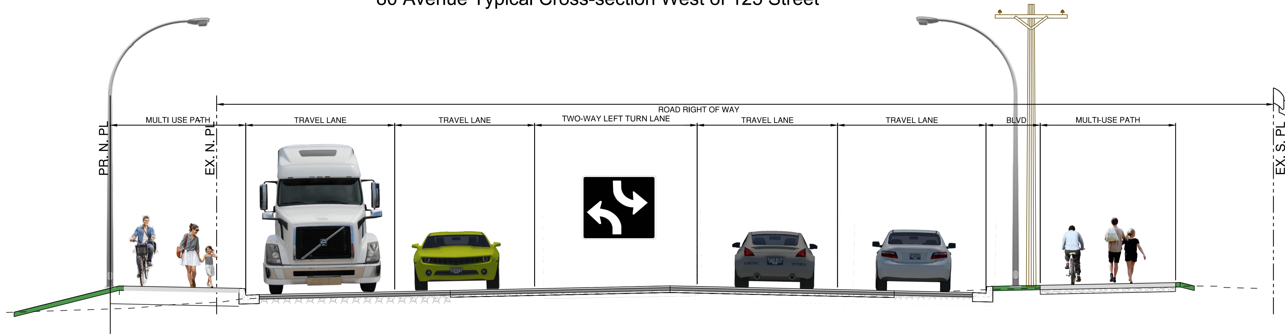
80 Avenue Typical Cross-section West of 125 Street
