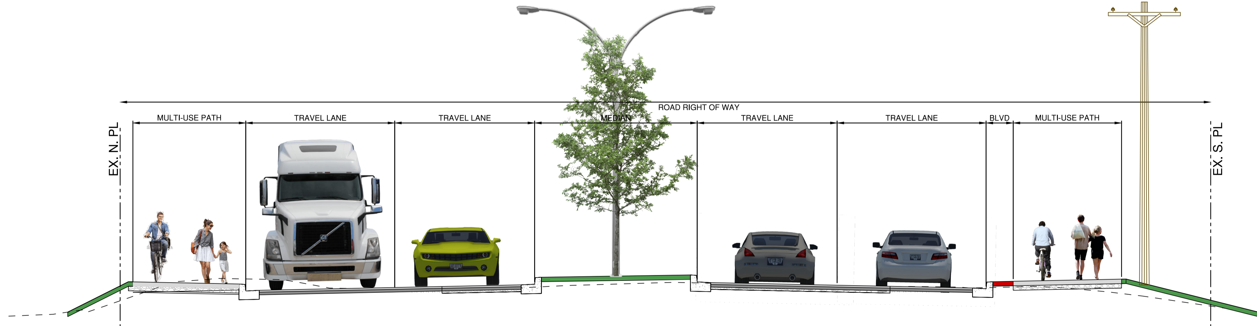
80 Avenue Typical Cross-section East of 122 Street
