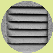
Carbon monoxide
