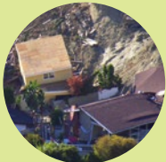
Landslides
