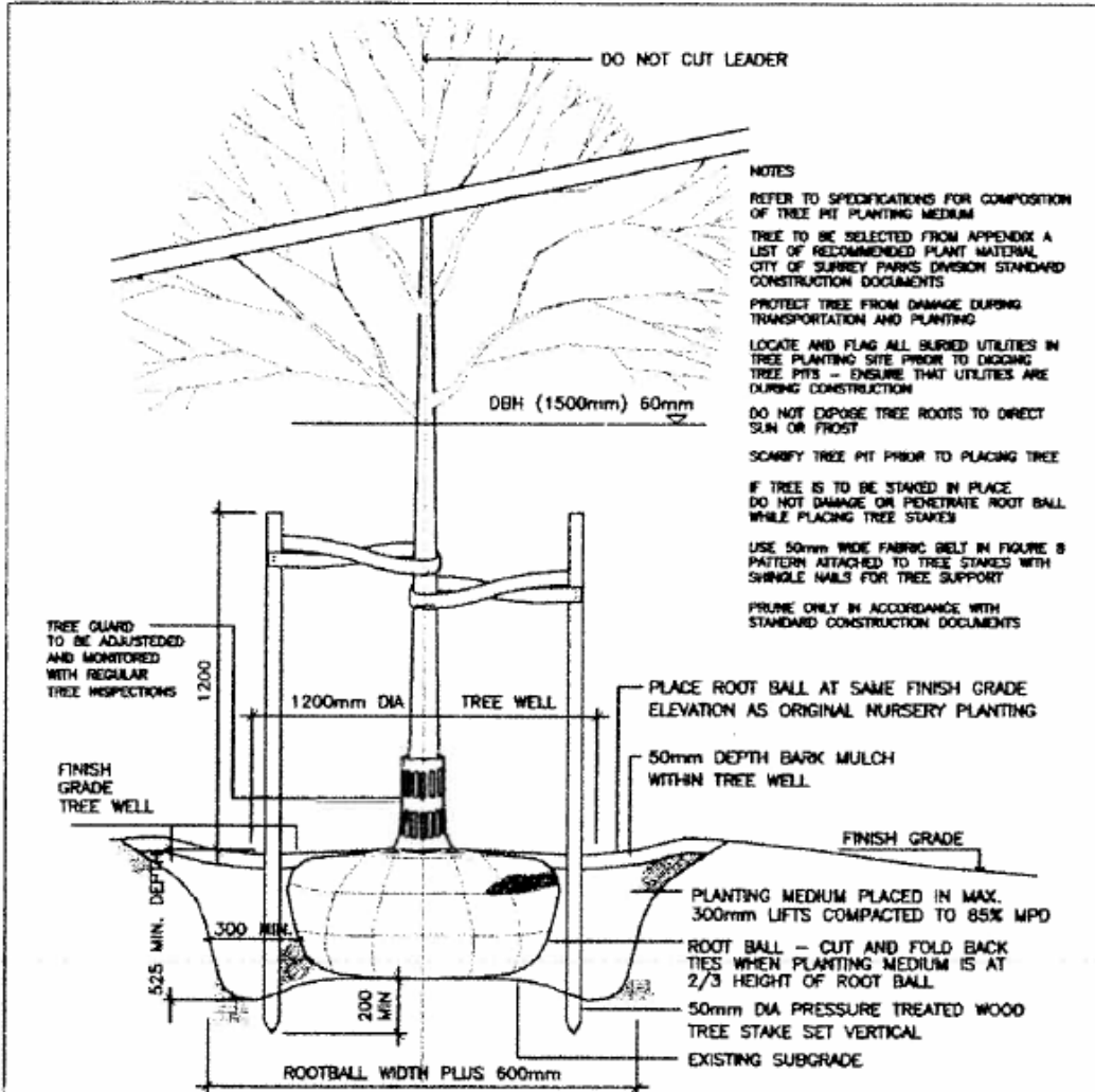
A TREE PLANTING - RESIDENTIAL STREETS AND PARKS SCALE 1:30
