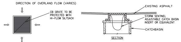
TYPICAL DETAIL OF CATCH BASIN SEDIMENT TRAP ON ASPHALT SURFACES N.T.S.
