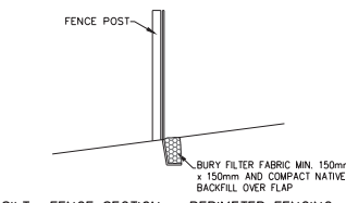
SILT - FENCE SECTION - PERIMETER FENCING N.T.S.
