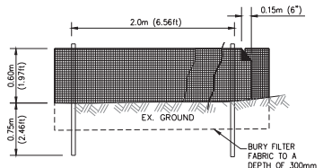
SILT - FENCE DETAIL - PERIMETER FENCING N.T.S.
