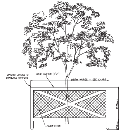
TREE PROTECTION FENCING DETAIL N.T.S.
